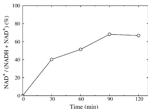
Fig. 5. Generation of NAD + by oxidation of NADH. The NAD + /NADH concentrations and ratios were measured using an NAD + /NADH assay kit. The absorbance at 570 nm was measured until 120 min after 5 \mu M CP-Pt were added to the 5 \mu M NADH solution. Values represent means \pm S.D. of three experiments. When not shown, deviations lie within the symbols.
