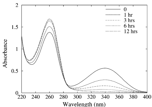
Fig. 2. Time-dependent change in absorption spectra. CP-Pt were incubated with NADH in water at room temperature for the indicated times. The concentrations of platinum in CP-Pt and NADH were 50 and 100 \mu\text{M} , respectively.
