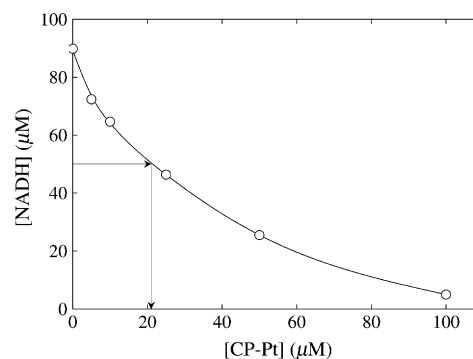
Fig. 4. Dose-dependent decrease in NADH. The absorption band at 340 nm was monitored for 3 h after CP-Pt were added to a 100- \mu\text{M} NADH solution. The concentration of platinum in CP-Pt was altered from 5 to 100 \mu\text{M} . Values represent means \pm S.D. of five experiments. When not shown, deviations lie within the symbols.
