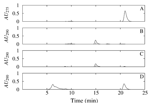
Fig. 8. HPLC analysis of CoQ 1 . Twenty microliters of 0.25 mM CoQ 1 in the HEPES/OH buffer was injected into the HPLC (A). After a 1 h reduction with 4 mM borohydride, 20 \mu l of 0.25 mM CoQ 1 was injected (B). After a 1 h incubation with 0.25 mM CP-Pt at room temperature, 20 \mu l of the consequent mixture containing 0.25 mM CoQ 1 was injected (C). The concentration of ferricyanide was 4 mM, and the incubation time was 1 h (D). The 275 nm band is plotted in panel A, and the 290 nm band is plotted in panels (B–D). AU: absorbance unit.
