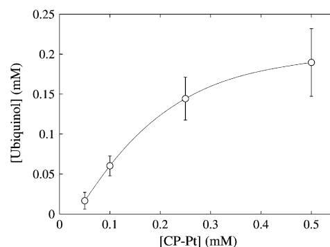
Fig. 9. Dose-dependent reduction of CoQ 1 by CP-Pt. CoQ 1 at 0.25 mM was incubated with 0.05, 0.1, 0.25, and 0.5 mM CP-Pt at room temperature for 15 min and detected at 290 nm with the HPLC system. The concentrations of reduced CoQ 1 were calculated as described in the Section 2. Values represent means \pm S.D. of three experiments. When not shown, deviations lie within the symbols.
