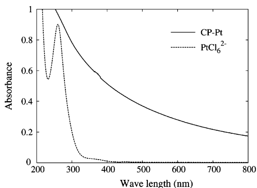
Fig. 1. UV-vis absorption spectra of platinum nanoparticles protected with citrate and pectin (CP-Pt) and aqueous hexachloroplatinate ( \text{PtCl}_6^{2-} ) from 200 to 800 nm. The concentrations of platinum as CP-Pt and as \text{PtCl}_6^{2-} were 200 and 50 \mu\text{M} , respectively.
