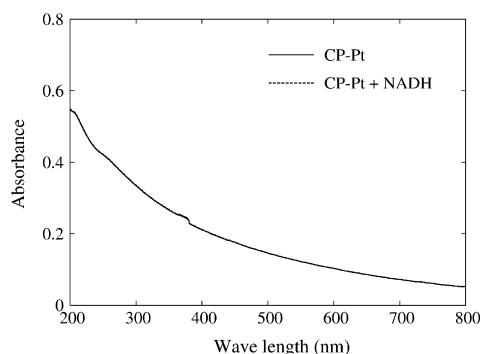
Fig. 6. UV-vis surface plasmon absorption spectra of CP-Pt after NADH oxidation. CP-Pt was incubated with NADH in water at room temperature for 2 h. The concentrations of platinum in CP-Pt and NADH were 100 \mu M and 200 \mu M, respectively. After 2 h reaction, the incubated mixture was centrifuged by Amicon Ultra centrifugal filter devices to remove NADH and NAD and then re-dispersed with the equal volume of water. This washing process was repeated 10 times. For control, we used CP-Pt subjected to 2 h incubation without NADH and following series of washing. The spectrum measurements were independently repeated three times. A representative set of spectra were shown.
