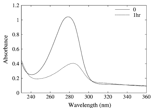
Fig. 7. The absorption change of CoQ 1 . The CP-Pt were mixed with CoQ 1 in 140 mM KCl and 10 mM HEPES/OH, pH 7.5 (HEPES/OH buffer). Their final concentrations were 250 and 50 \mu M, respectively. The resultant mixture was incubated for 1 h at room temperature under an N 2 atmosphere.
