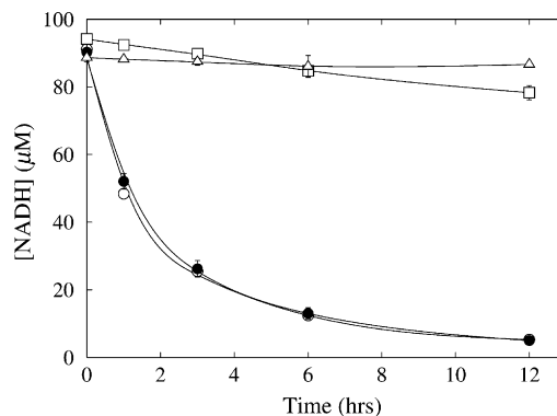
Fig. 3. Oxidation of NADH by platinum only. CP-Pt were incubated with NADH in water at room temperature for predetermined periods (open circle). The concentrations of platinum in CP-Pt and NADH were 50 and 100 \mu\text{M} , respectively, at the start of incubation. A similar experiment was performed under an \text{N}_2 atmosphere (closed circle). Auto-oxidation of NADH was monitored by incubating 100 \mu\text{M} NADH alone (open square). To examine whether the protecting reagents of CP-Pt oxidize NADH, citrate and pectin were incubated with NADH (open triangle). The concentrations of citrate and pectin were 10 mM and 0.60 mg/ml, respectively. The concentrations of NADH were calculated using the \epsilon value of 6.22 \text{ mM}^{-1} \text{ cm}^{-1} [18]. Values represent means \pm S.D. of five experiments. When not shown, deviations lie within the symbols.
